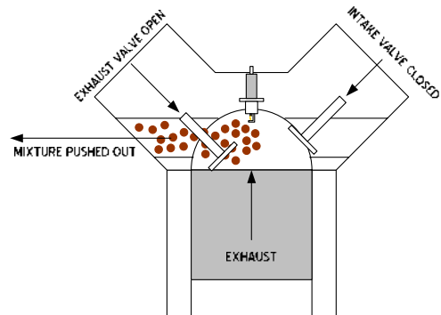
Figure 41.4: Exhaust
