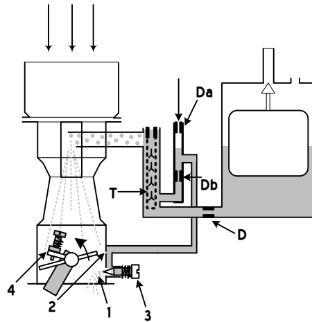
Figure 4: Idle Speed Circuit. D main fuel jet, Da idle speed air jet, Db idle speed fuel jet, 1 idle speed mixture orifice, 2 transition device, 3 idle speed mixture adjusting screw, 4 throttle setting or idle speed adjusting screw
