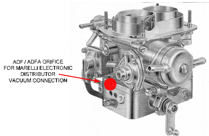
Figure 47: Location of port for vacuum advance
