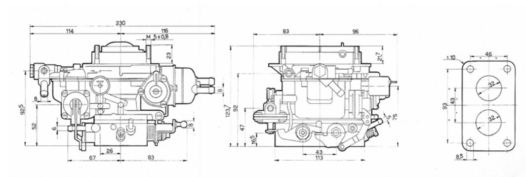
Figure 32: ADF Dimensions
