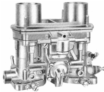
Figure 14: IDF Carburetor Side View
