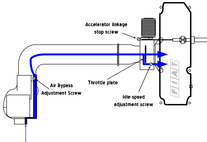
Figure 36: Idle Speed Control in the Bosch L-Jetronic System
