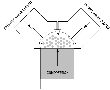
Figure 41.2: Compression
