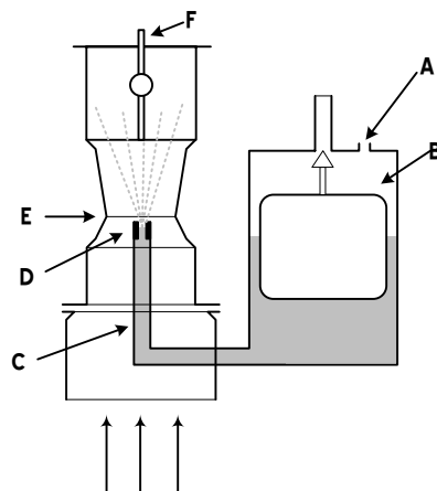
Figure 2: Updraft Carburetor. A Float Chamber Vent, B Fuel Bowl or Chamber, with Float, C Spray Tube, D Fuel Jet, E Venturi, F Throttle
