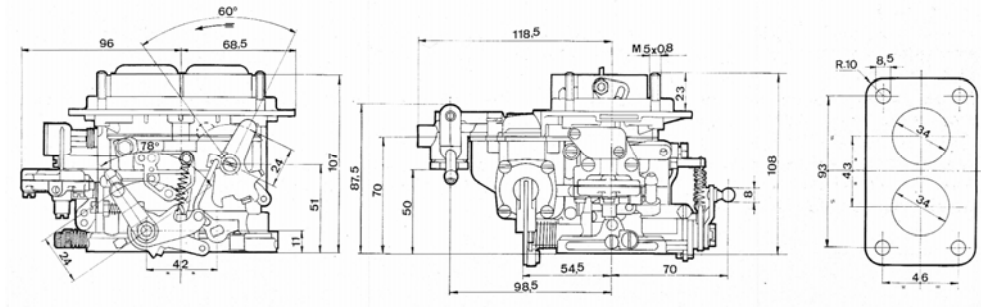
Figure 25: DMS Dimensions
